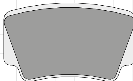
DP990 58.8 x 35.1 x 8.3mm
