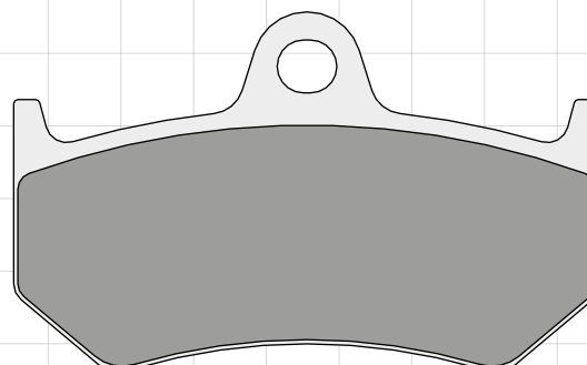
DP994 69.8 x 42.6 x 7.5mm
