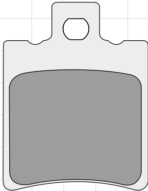
DP634 39.8 x 51.2 x 6.4mm
