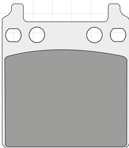
DP916 57.6 x 65.2 x 11.0mm
