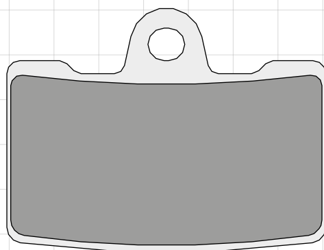
SDP993 61.6 x 47.6 x 7.7mm
