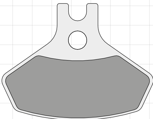
DP991 67 x 51.9 x 7.6mm
