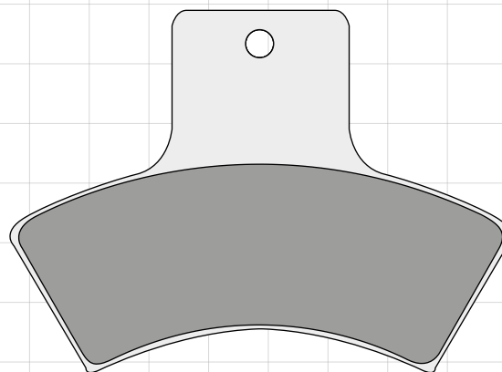
DP915 73 x 53.2 x 7.0mm
