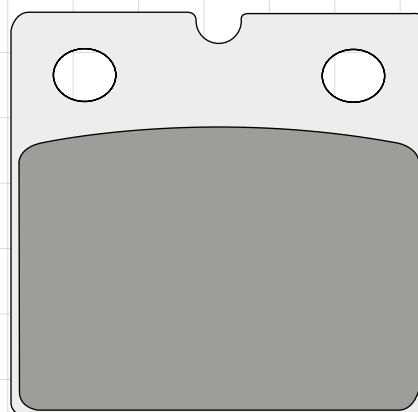
DP701 55.5 x 54. x 9.0mm
