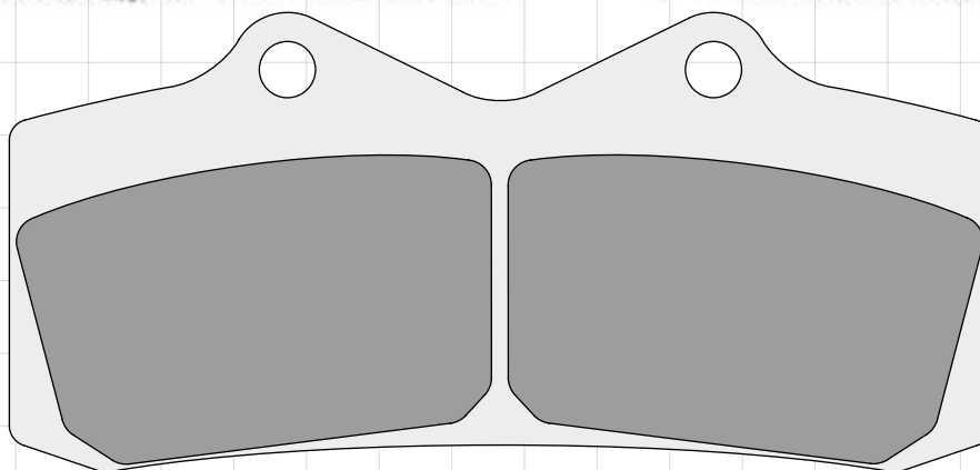
DP529 117.1 x 54.8 x 8.0mm
