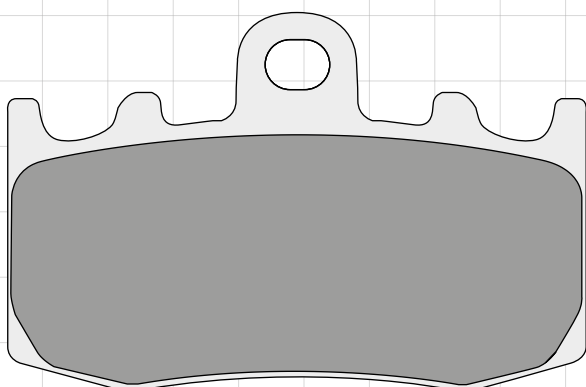
DP641 77.3 x 50.3 x 8.6mm
