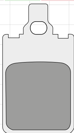
DP610 31.7 x 57 x 5.6mm
