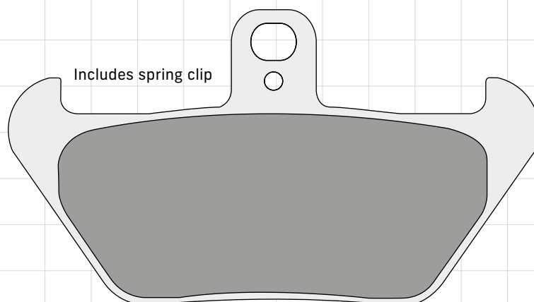
DP615 100 x 56 x 8.3mm
