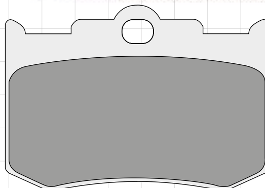
RDP913 69.4 x 48.8 x 10.5mm
