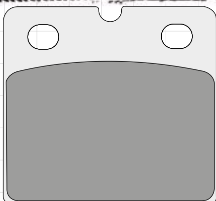
DP608 57.8 x 53.4 x 9.0mm
