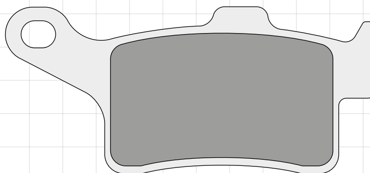
DP533 96.4 x 43.6 x 8.0mm
