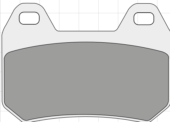
DP637 75.2 x 53.5 x 8.7mm
