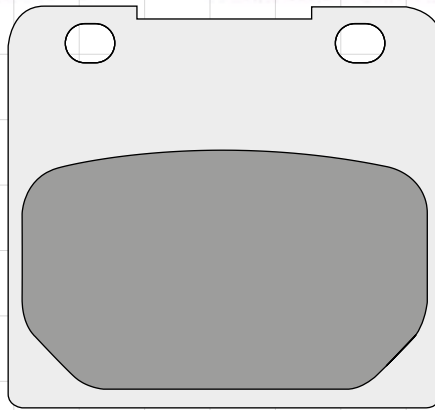
DP210 57.9 x 53.6 x 8.7mm
