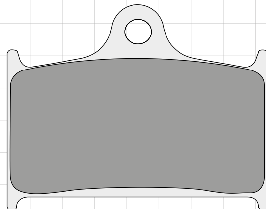
DP213 69.7 x 55.5 x 8.5mm
