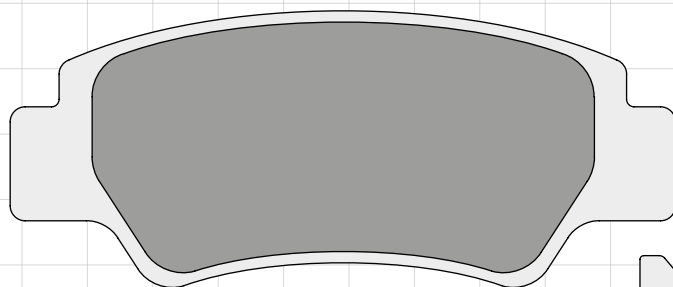
DP702 88.8 x 36.9 x 10.8mm
