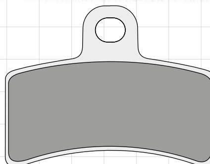
DP640 56.75 x 43.4 x 6.4mm
