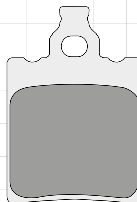
DP611 36 x 52 x 6.4mm
