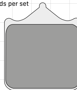
DP638 35 x 40.5 x 7.5mm
