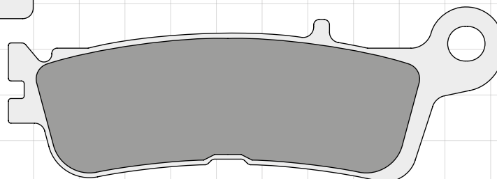
DP703 94 x 33.3 x 7.5mm
