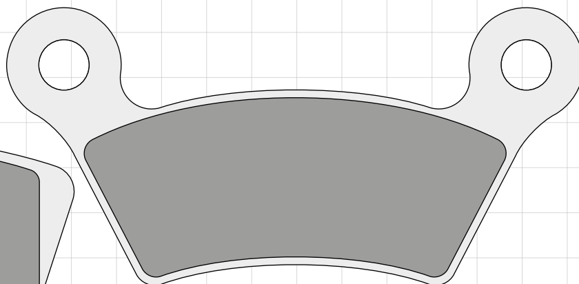
DP532 110.9 x 53.4 x 7.9mm
