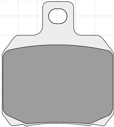
DP631 50.8 x 56.4 x 7.9mm
