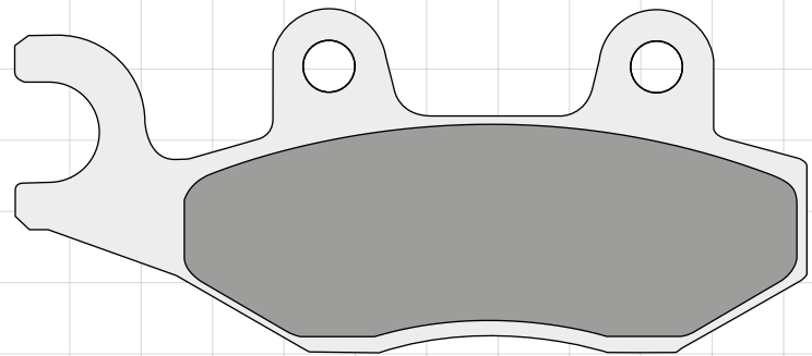
DP211 77 x 42 x 7.6mm 96.7 x 42 x 7.6mm
